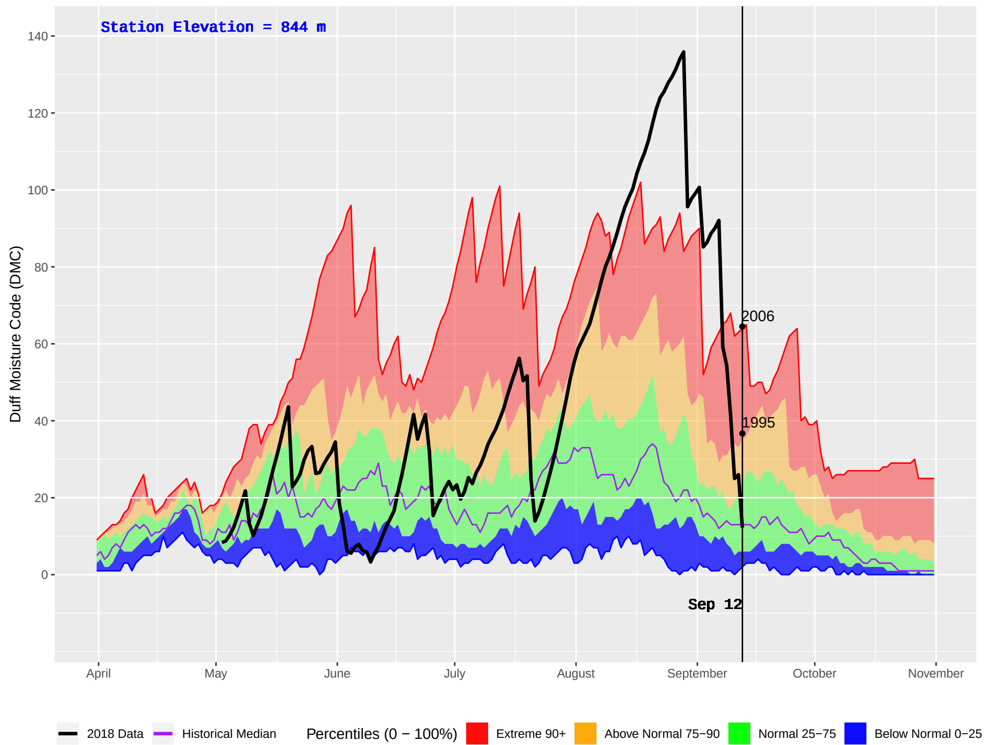
GANOKWA (182) : Historical (1993–2016) and Current (2018) Daily Duff Moisture Code (DMC)
