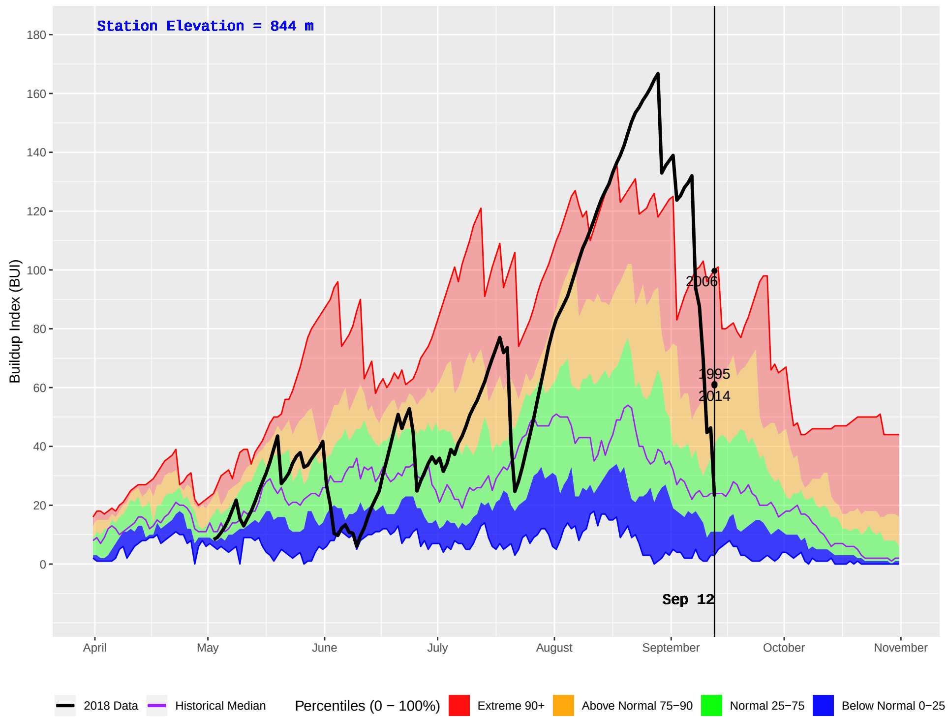
GANOKWA (182) : Historical (1993–2016) and Current (2018) Daily Buildup Index (BUI)
