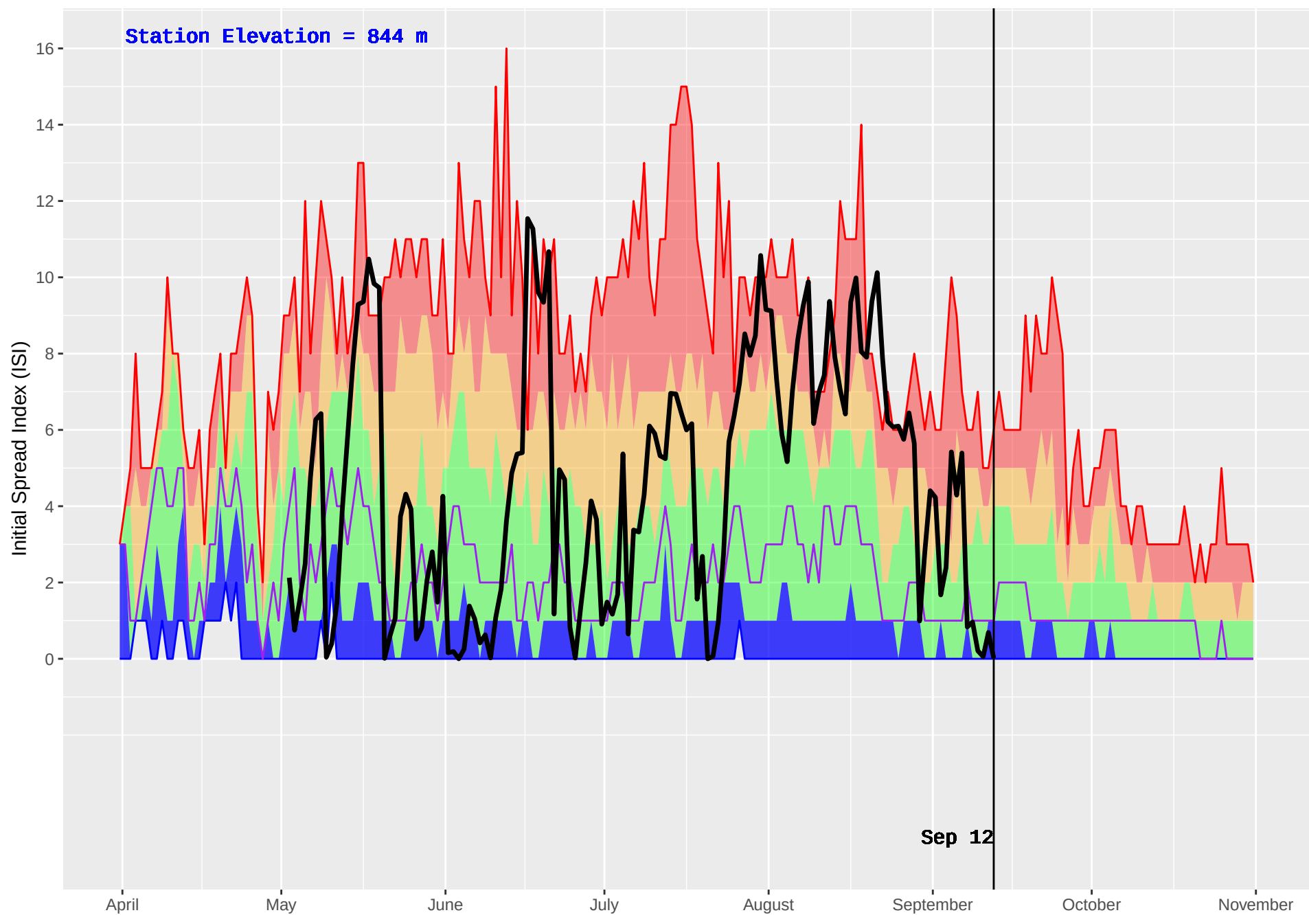
GANOKWA (182) : Historical (1993–2016) and Current (2018) Daily Initial Spread Index (ISI)
