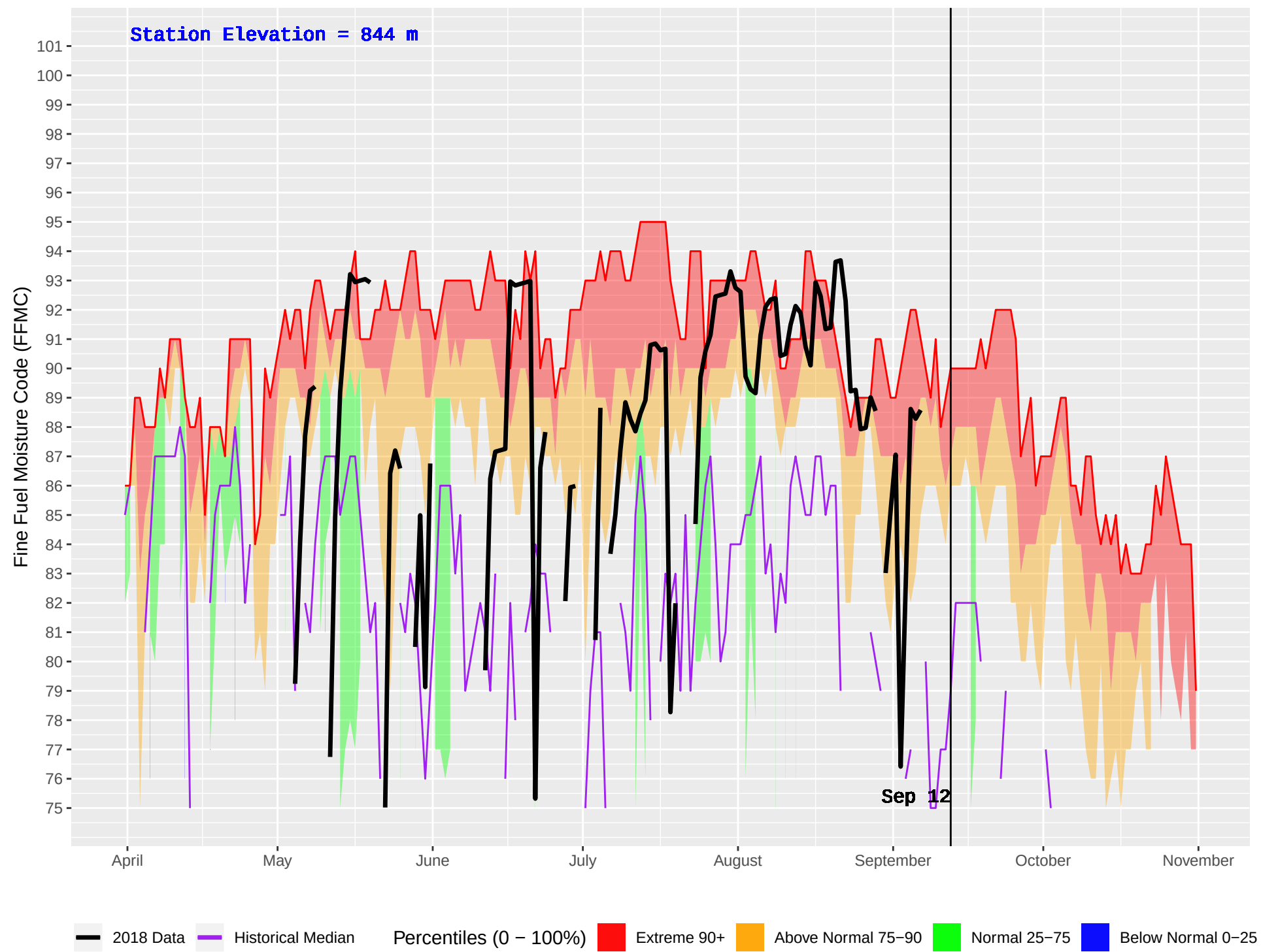
GANOKWA (182) : Historical (1993–2016) and Current (2018) Daily Fine Fuel Moisture Code (FFMC)
