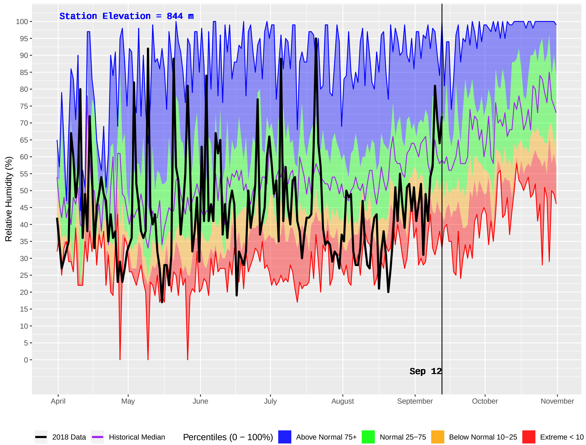
GANOKWA (182) : Historical (1993–2016) and Current (2018) Daily Relative Humidity
