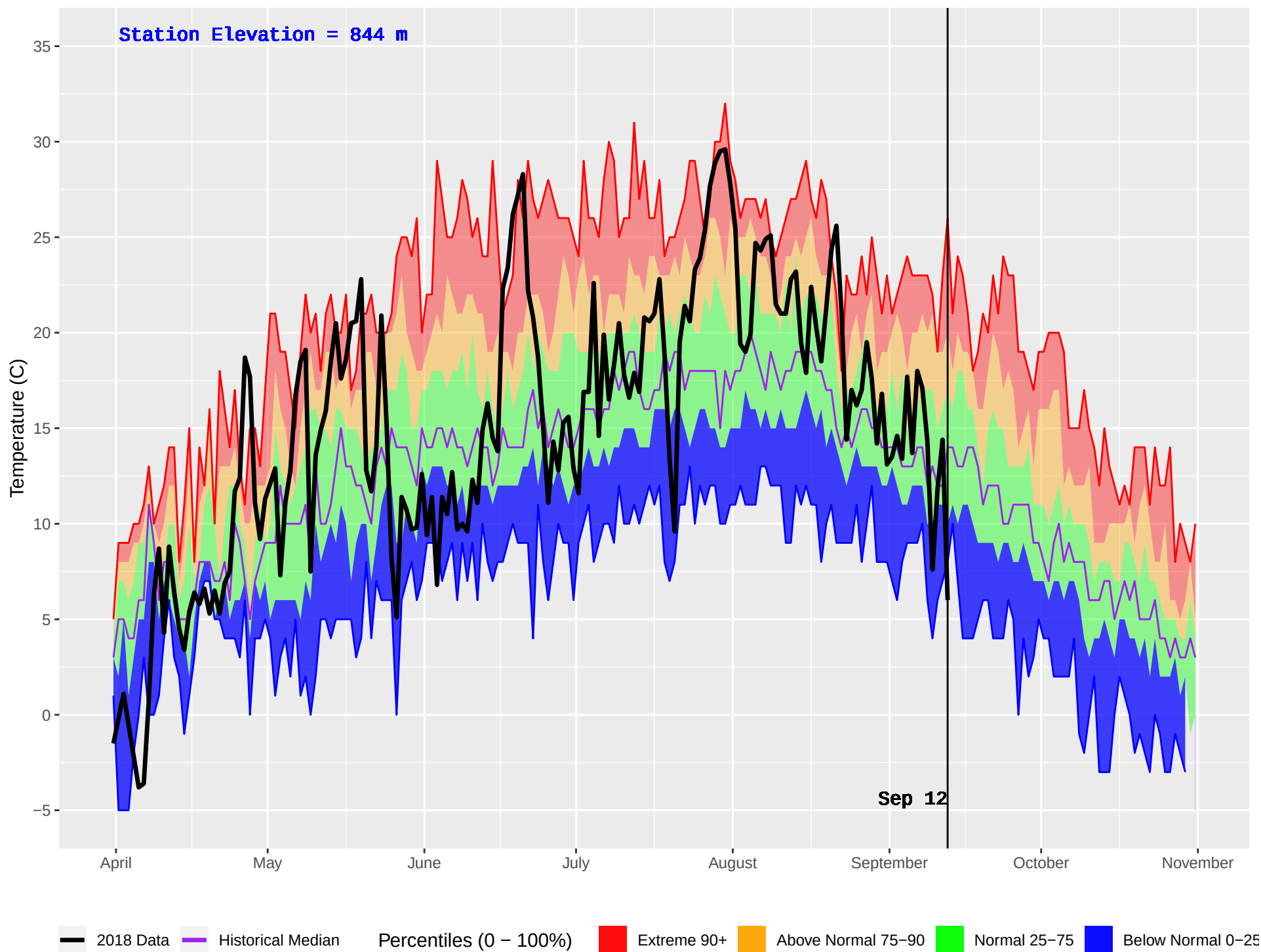
GANOKWA (182) : Historical (1993–2016) and Current (2018) Daily Temperature
