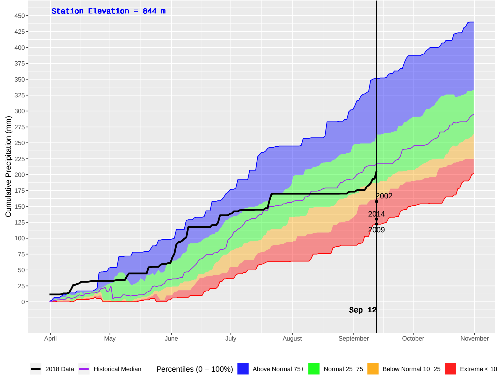
GANOKWA (182) : Historical (1993–2016) and Current (2018) Daily Cumulative Precipitation
