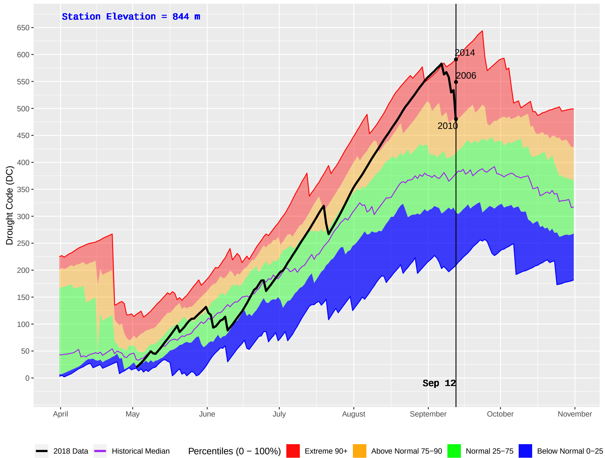
GANOKWA (182) : Historical (1993–2016) and Current (2018) Daily Drought Code (DC)
